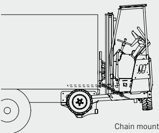
Chain mount
